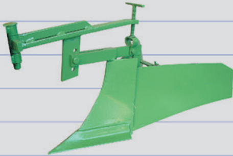
ARATRO ASSOLCATORE-RINCALZATORE MOTOR-CULTIVATOR WITH RIDGER ΑΥΛΑΚΩΤΗΡΑΣ ΔΙΠΤΕΡΟΣ
