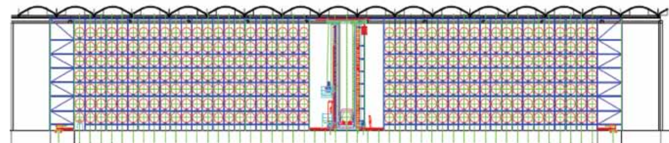
Paper rolls stored in double and triple depth for volume maximization
