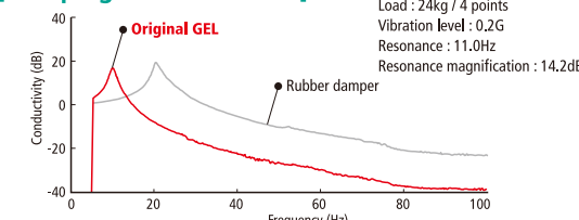
[Damping Characteristics]
