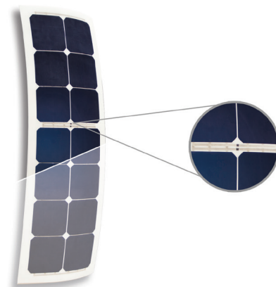
Custom panel with laminated bypass diodes, to minimize shading effects on a flexible panel without junction box
