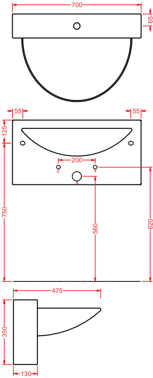
WLL002 WALL lavabo sospeso wall-hung washbasin
